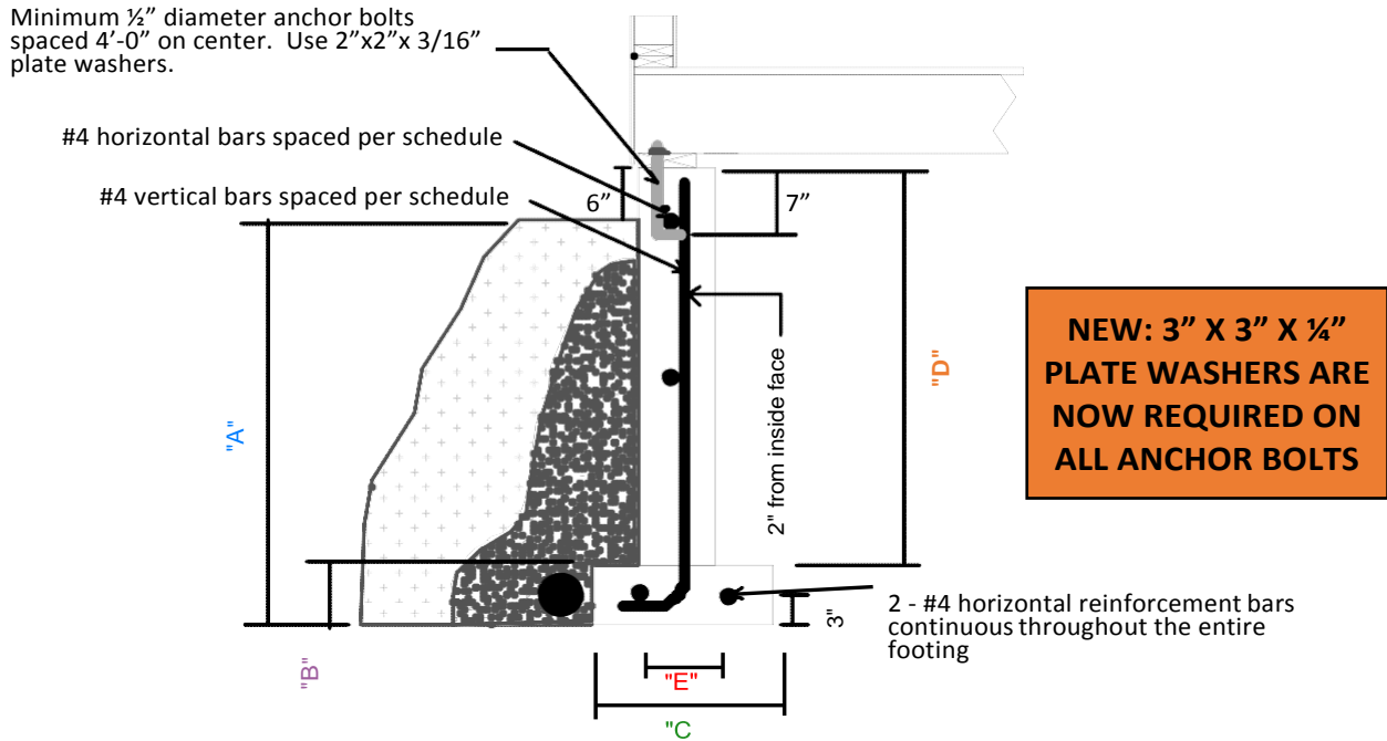
FIGURE 1 – PRESCRIPTIVE FOUNDATION REQUIREMENTS
