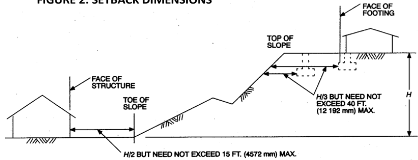
FIGURE 2: SETBACK DIMENSIONS
